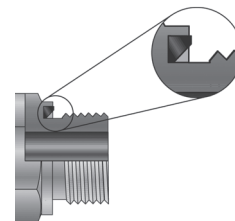
Fig. E6 — O-Ring in Fitting Groove
