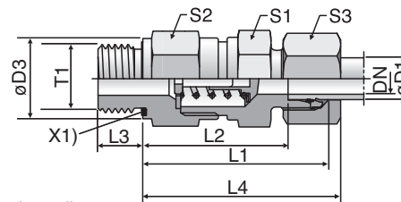
X1) Elastic sealing
