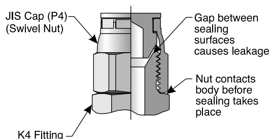
Fig. H5 – Illustration Showing Potential Leakage Problem When Mixing JIS and K4 Components
