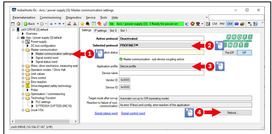
Fig. 7-17: Activating PROFINET®
