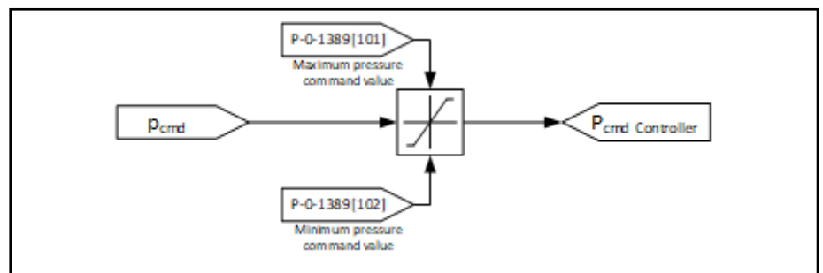
Fig. 6-6: Limitation of pressure command value
