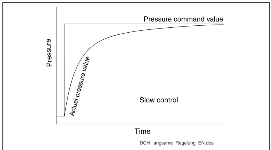
Fig. 7-53: Slow control
