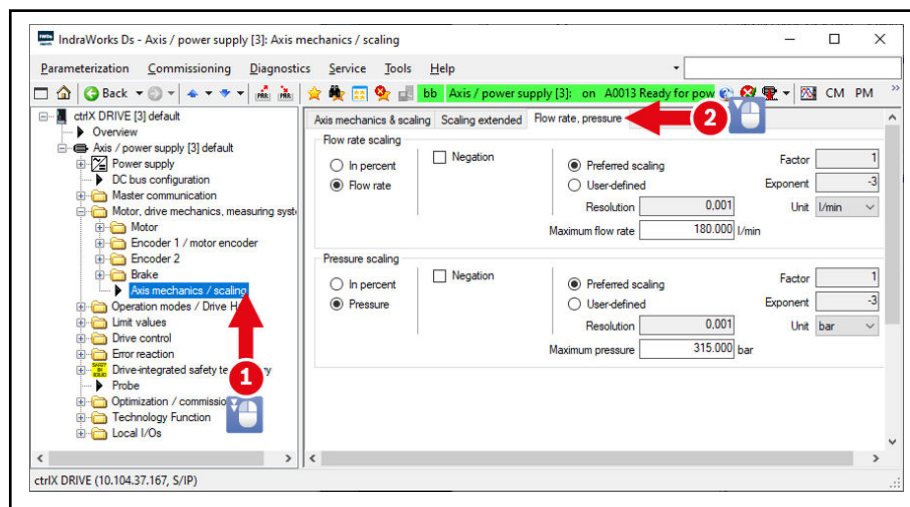
Fig. 7-23: Scaling of flow and pressure
