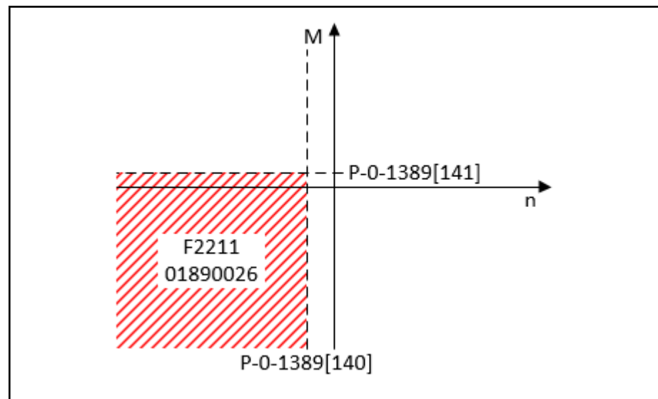
Fig. 7-70: Monitoring for an inadmissible operating point
