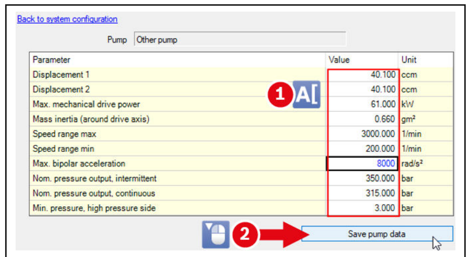
Fig. 7-30: Configuring pump data of a user-defined pump
