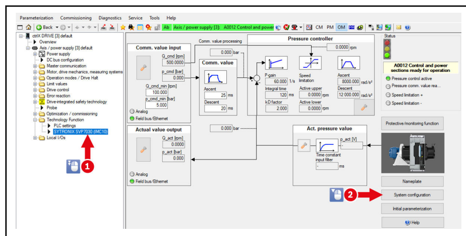
Fig. 7-43: System configuration
