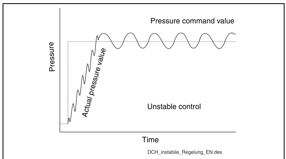
Fig. 7-54: Unstable control
