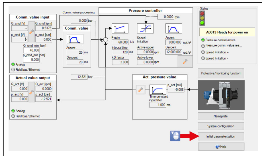
Fig. 7-31: Initial parameterization
