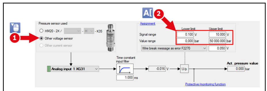
Fig. 7-41: Selection of another voltage sensor
