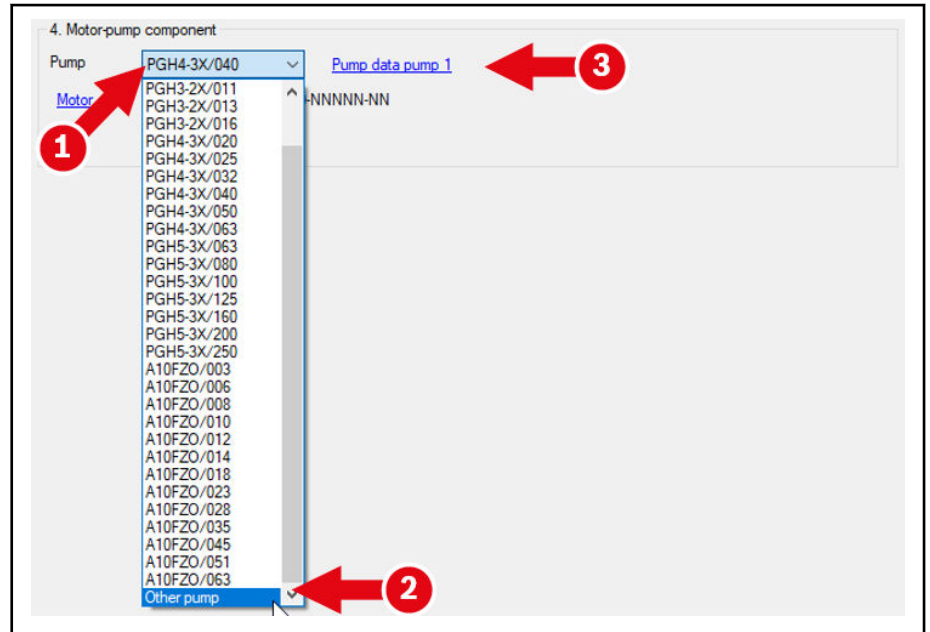
Fig. 7-29: Setting a user-defined pump
