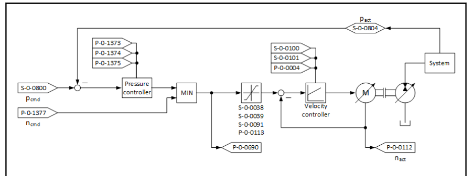
Fig. 6-1: Controller structure for p/Q control in the open circuit
