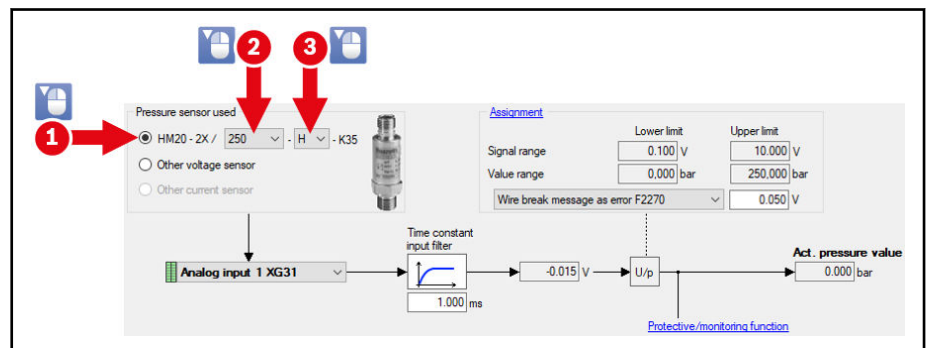
Fig. 7-40: Selection of the voltage sensor HM20-2X/...
