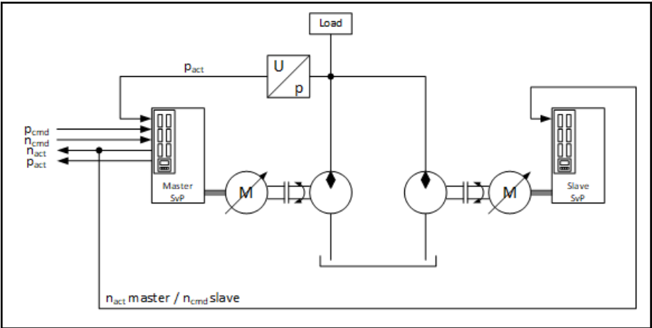
Fig. 6-13: Schematic circuit without check valve at the slave pump
