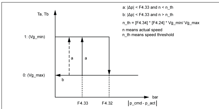
Fig. 7-6: Action logic of relay
