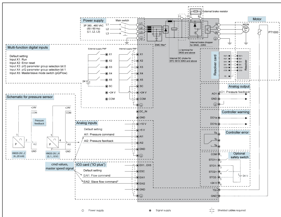
Fig. 6-1: Example wiring diagram with Rexroth MS2N motor analog set point control scheme
