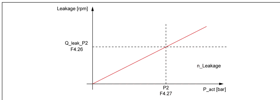
Fig. 7-9: Leakage compensation
