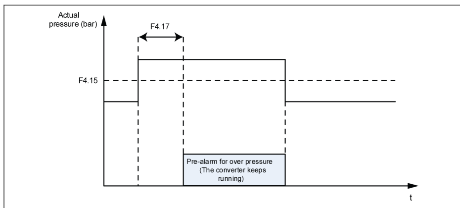
Fig. 7-12: F4.15 maximum system pressure warning
