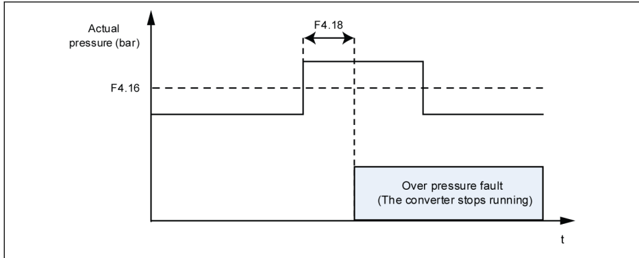
Fig. 7-13: F4.16 maximum pump pressure fault
