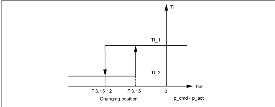
Fig. 7-3: p/Q PID integrator switching
